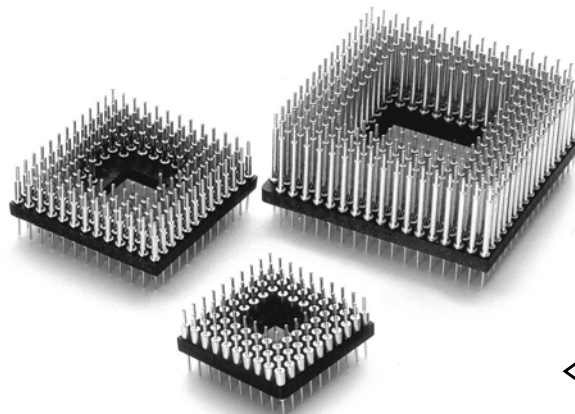
HEADER PIN TYPE 5012 SERIES 550
