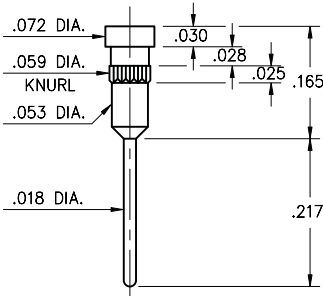
1940-0-00-XX-00-00-03-0 Press-fit in .057 mounting hole
