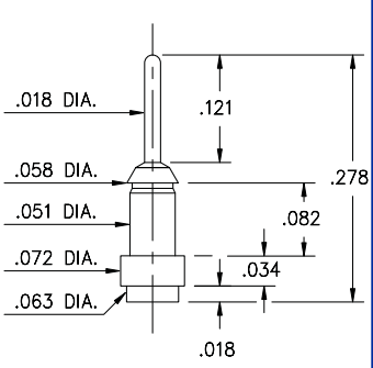
2956-1-00-XX-00-00-03-0 Surface mount
