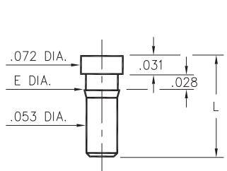
02XX-0-00-XX-00-00-03-0 Press-fit in .057/.059 mounting hole
