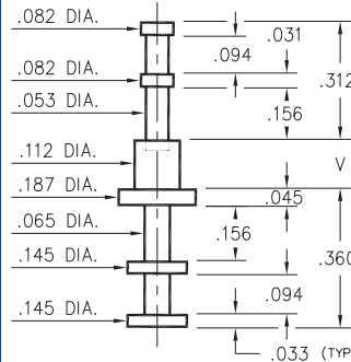
2812-X-00-XX-00-00-07-0 Swage mount in .116 hole
