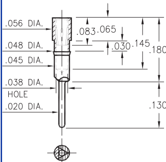
1782-0-15-XX-43-XX-04-0 Press-fit in .045 mounting hole
