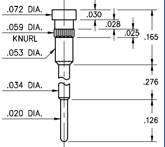
1938-0-00-XX-00-00-03-0 Press-fit in .057 mounting hole
