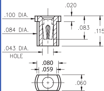
3907-0-18-XX-30-XX-10-0 Surface mount Also available on 12mm wide carrier tape: 4,000 parts per 13" reel. Order as: 3907-0-58-XX-30-XX-10-0
