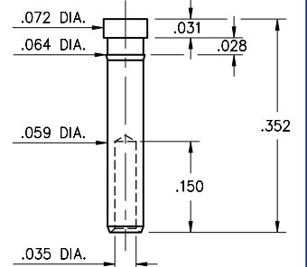
3000-0-00-XX-00-00-03-0 Press-fit in .061 mounting hole
