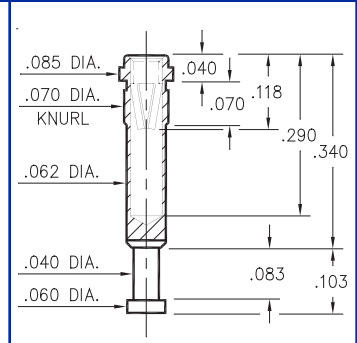
8864-0-15-XX-06-XX-10-0 Press-fit in .067 mounting hole
