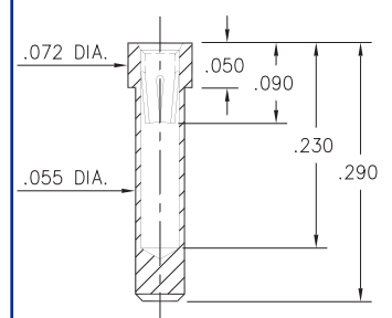
8363-0-15-XX-35-XX-10-0 Solder mount in .057 min. mounting hole
