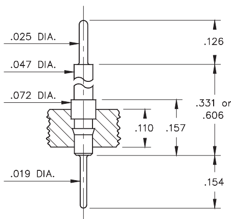
HEADER PIN TYPE 5504 & 5505 SERIES 551
