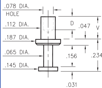
2805-X-00-XX-00-00-07-0 Swage mount in .116 hole
