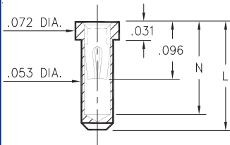
XXXX-0-15-XX-30-XX-10-0 Solder mount in .055 min. mounting hole
