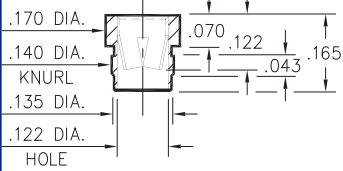
0388-0-15-XX-08-XX-10-0 Press-fit in .138 mounting hole
