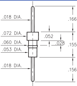
050X-0-00-XX-00-00-03-0 Press-fit in .057 mounting hole
