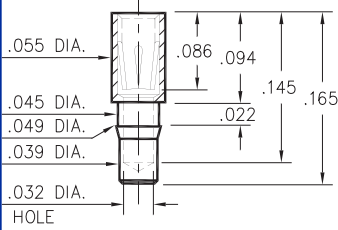
0385-0-15-XX-43-XX-10-0 Press-fit in .046 mounting hole
