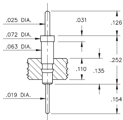
HEADER PIN TYPE 5503 SERIES 551
