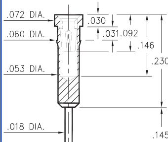
4001-0-15-XX-43-XX-04-0 Press-fit in .057 mounting hole
